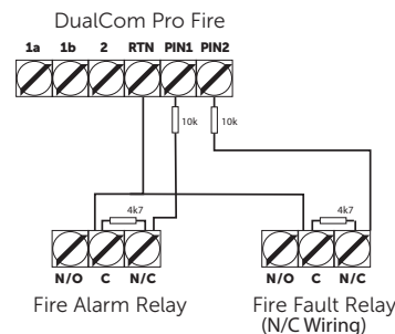
Normally closed wiring
