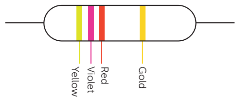
4k7/4.7k ohm resistor colour code
