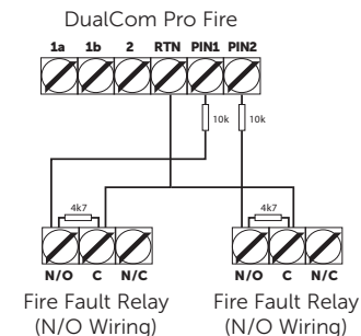
Normally open wiring
