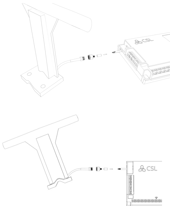
Figure 1 - Connection Examples
